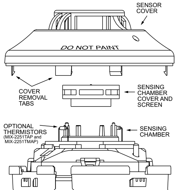
FIGURE 4. SENSOR ASSEMBLY:
